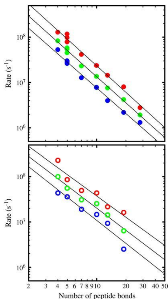
FIGURE 9 Temperature dependence of diffusion-limited rates in (top) 6 M GdmCl and (bottom) 8 M urea. The symbols are the values of \eta k_{D+} (solid circles, 6 M GdmCl; open circles, 8 M urea) at temperatures of 40°C (red), 20°C (green), and 0°C (blue) obtained from the analysis of the temperature- and viscosity-dependence of the measured rates (Table 3). The lines are linear regression fits to guide the eye. The apparent activation energies average 4.8 (\pm 0.4) \text{ kcal/mol} in 6 M GdmCl and 5.7 (\pm 0.7) \text{ kcal/mol} in 8 M urea.
